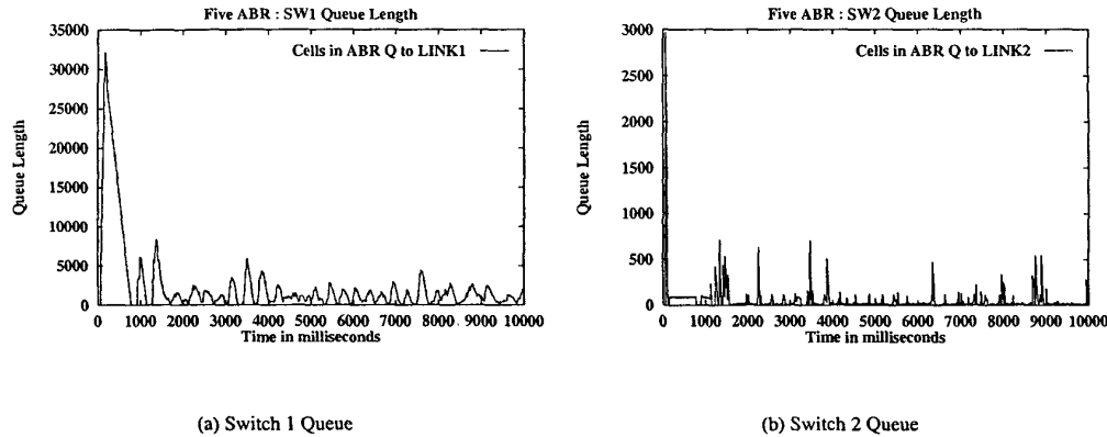
Fig. 10. Switch Queue Lengths for a 5-source LEO configuration
