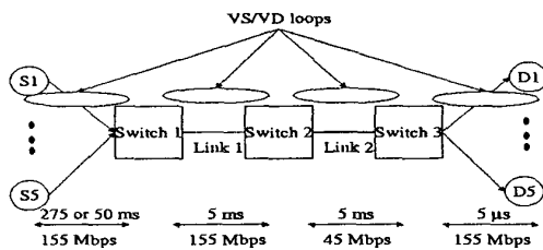
Fig. 9. Five source satellite configuration
