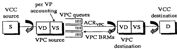
Fig. 7. Virtual source/virtual destination at the VPC end points
