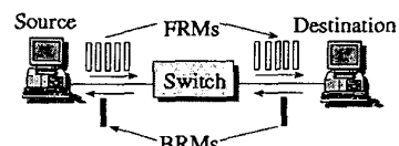
Fig. 3. Forward and backward RM cells flow in ABR connections
