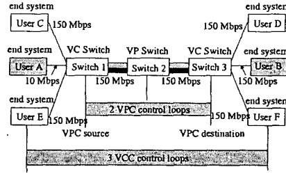
Fig. 5. Example 2: Two VPCs and multiple VCCs
