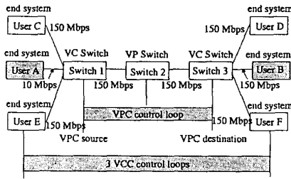
Fig. 4. Example 1: A single VPC and multiple VCCs
