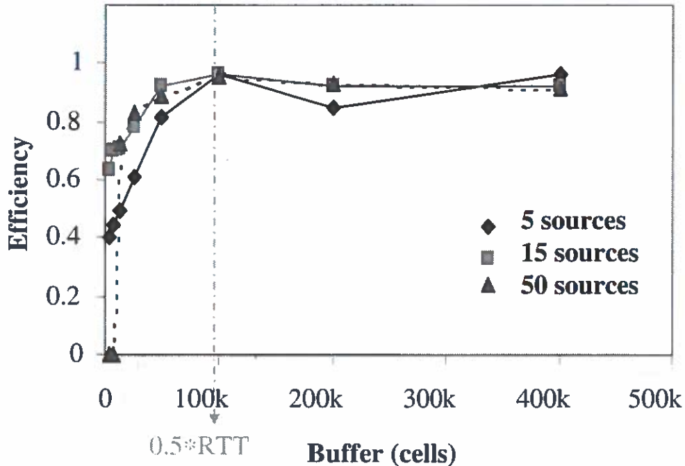
Figure 11.—TCP/IP UBR buffer requirements for single hop GEO.
