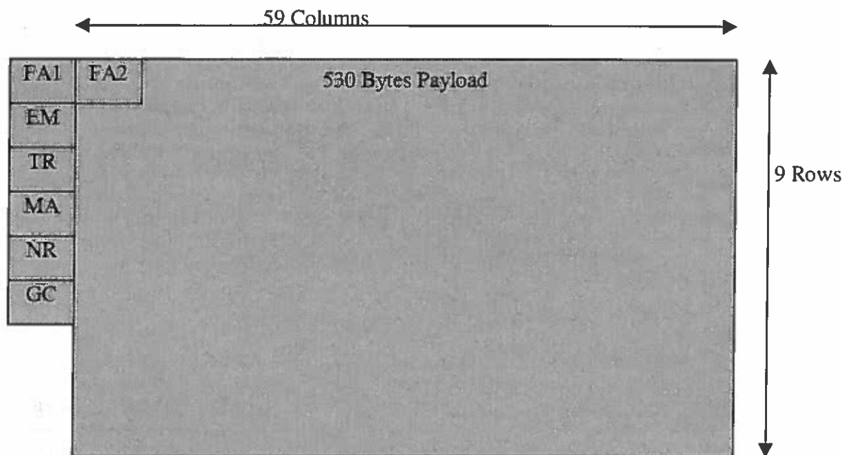
Figure 5.—34 Mbps PDH frames as specified in ITU-T G.832 [AGNE95].
