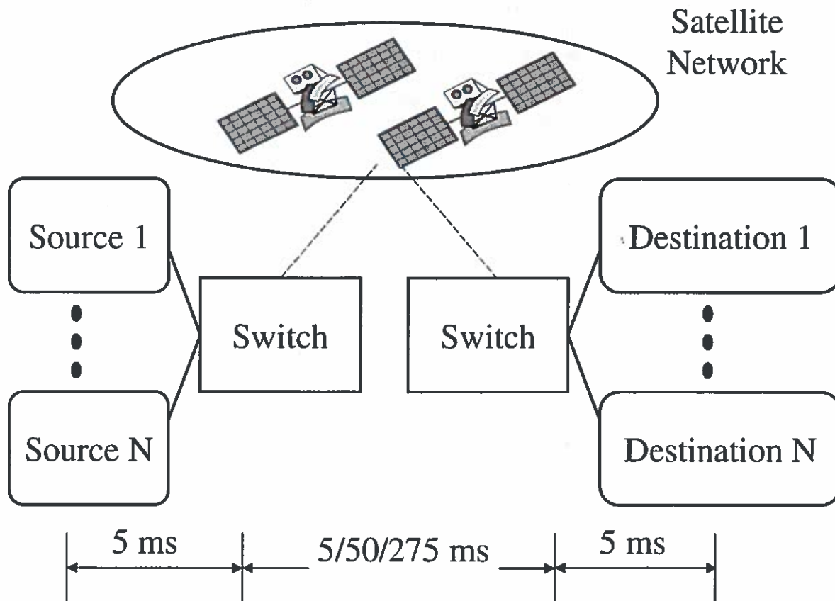
Figure 8.—Simulation model for TCP/IP over UBR.
