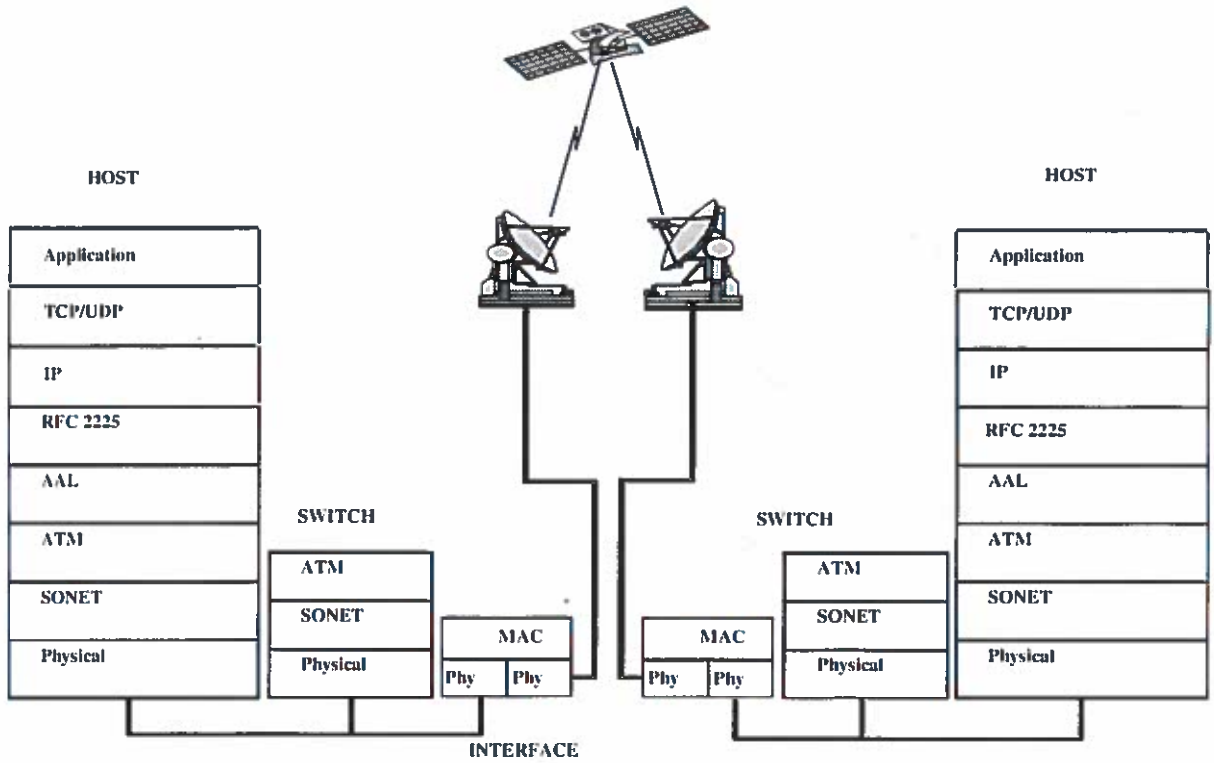
Figure 6.—Satellite ATM protocol stack.
