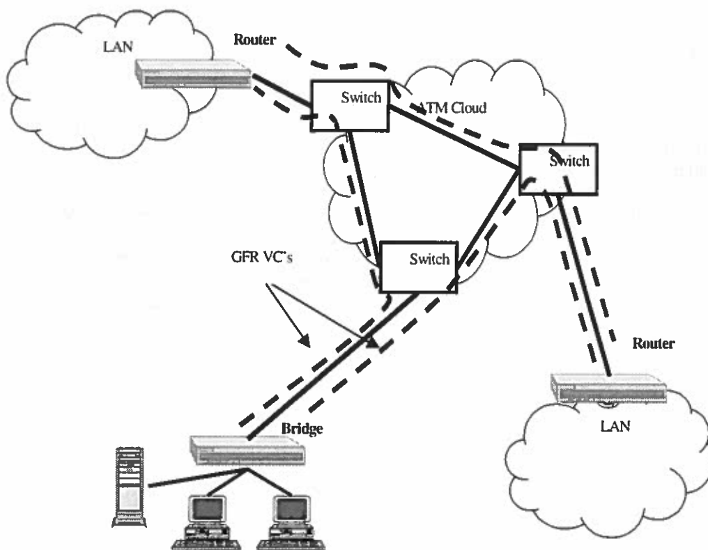
Figure 12.—GFR in ATM connected LAN's.
