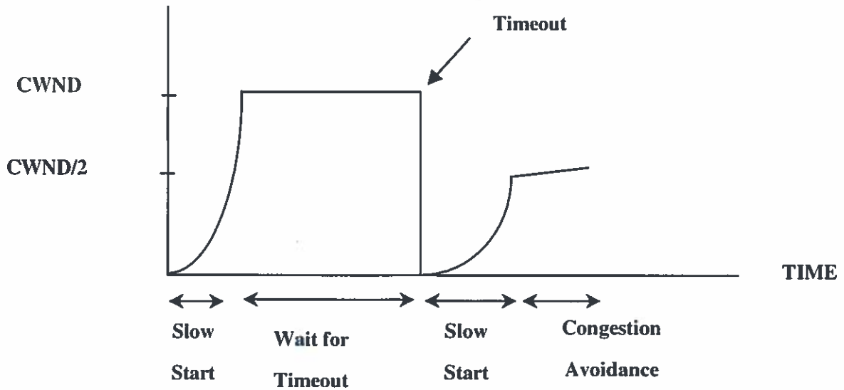
Figure 7.—TCP congestion control.
