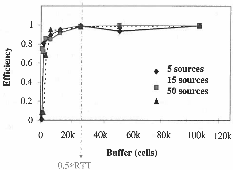
Figure 10.—TCP/IP UBR buffer requirements for multiple hop LEO.
