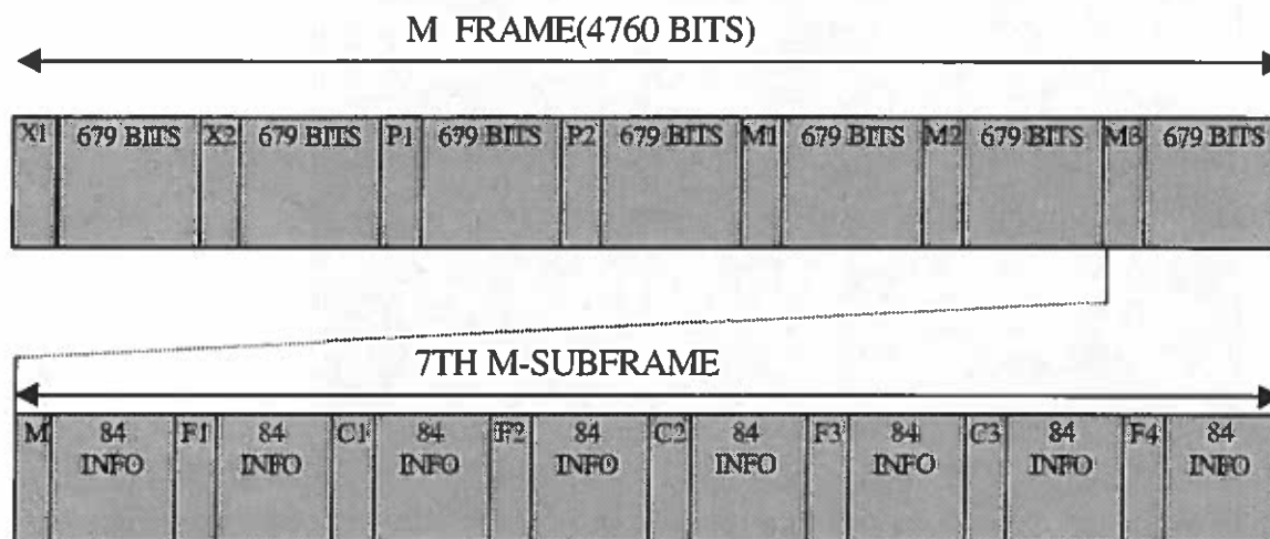
Figure 3.—DS3 signal format [CHIT94].
