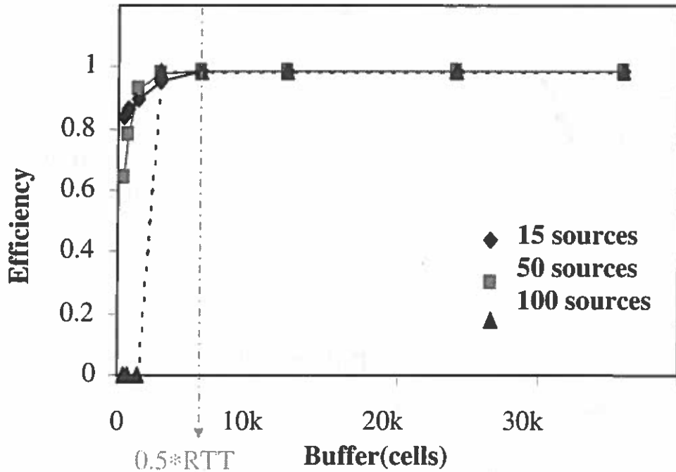
Figure 9.—TCP/IP UBR buffer requirements for single hop LEO.
