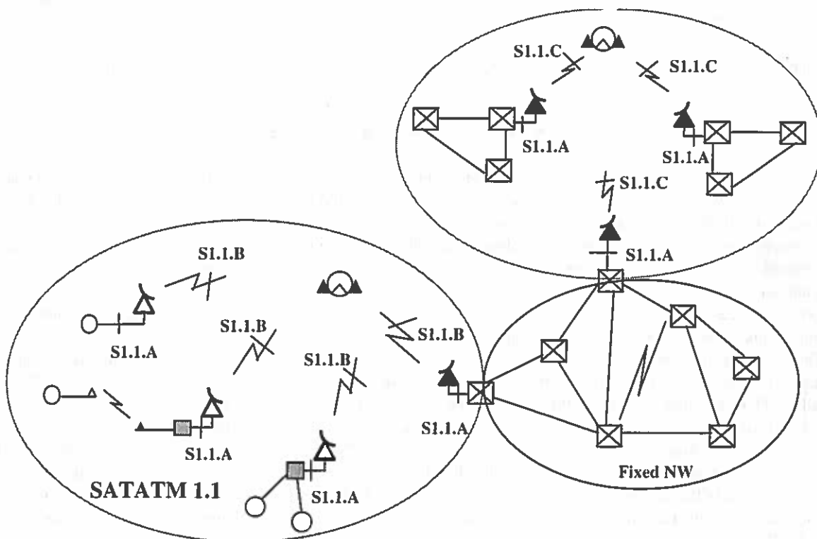
Figure 1.—SATATM 1.1, fixed ATM network access and network interconnect.
