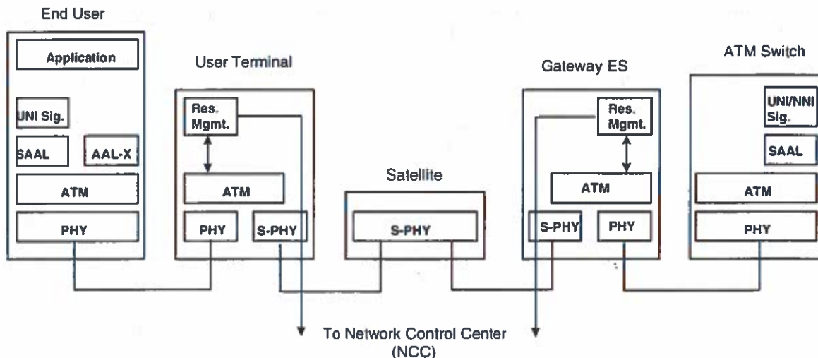
Figure 2.—SATATM 1.1, protocol reference model for network access.
