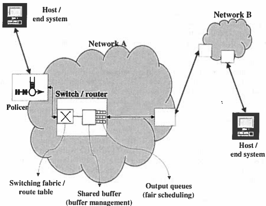
Figure 13.—Buffering, scheduling, and policing in the network.
