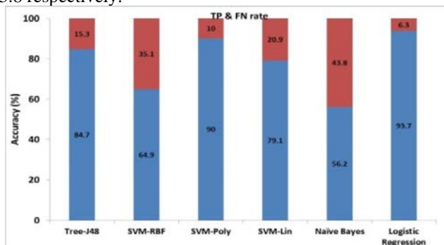
Fig. 2: TP and FN rate with UNSW dataset
