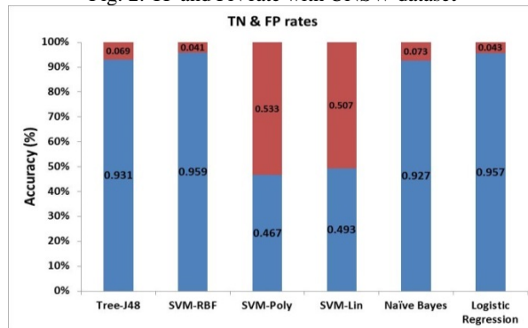
Fig. 3: TN and FP rate UNSW dataset
