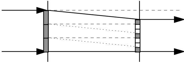
Figure A.3c: Input Rate < Output Rate, non-contiguous frame, zero-delay Switch
