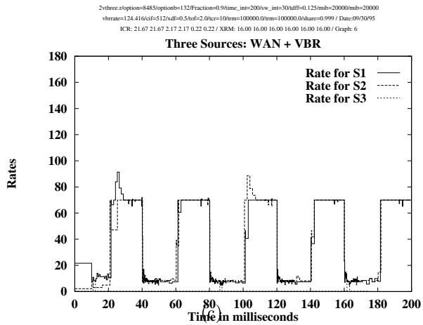
Figure 1: Three Source Configuration
