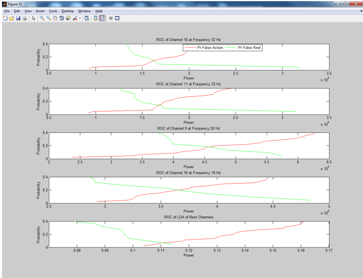
ROC Curves (zoomed in)
