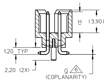
SECTION W-W
