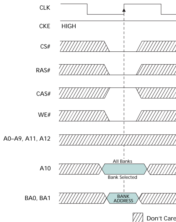
Figure 23: PRECHARGE Command
