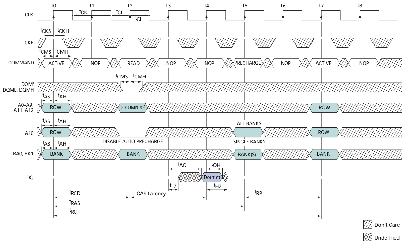
Figure 39: Single READ – Without Auto Precharge
