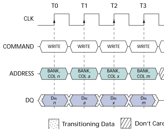
Figure 19: Random WRITE Cycles
