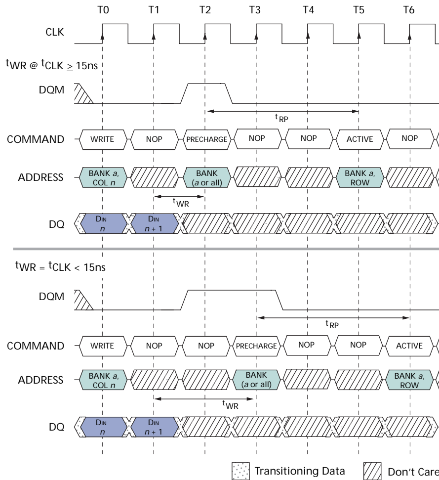
Figure 21: WRITE-to-PRECHARGE
