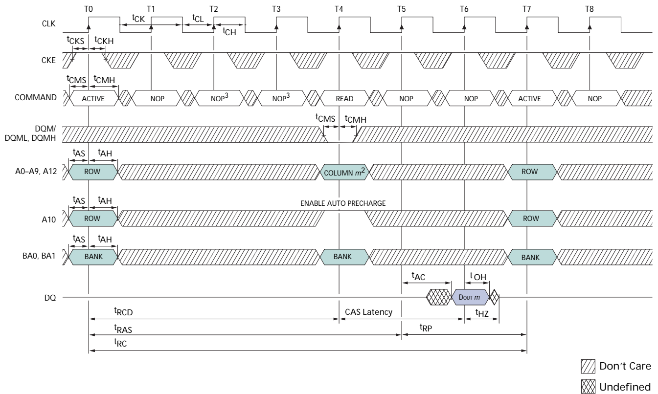
Figure 40: Single READ - with Auto Precharge
