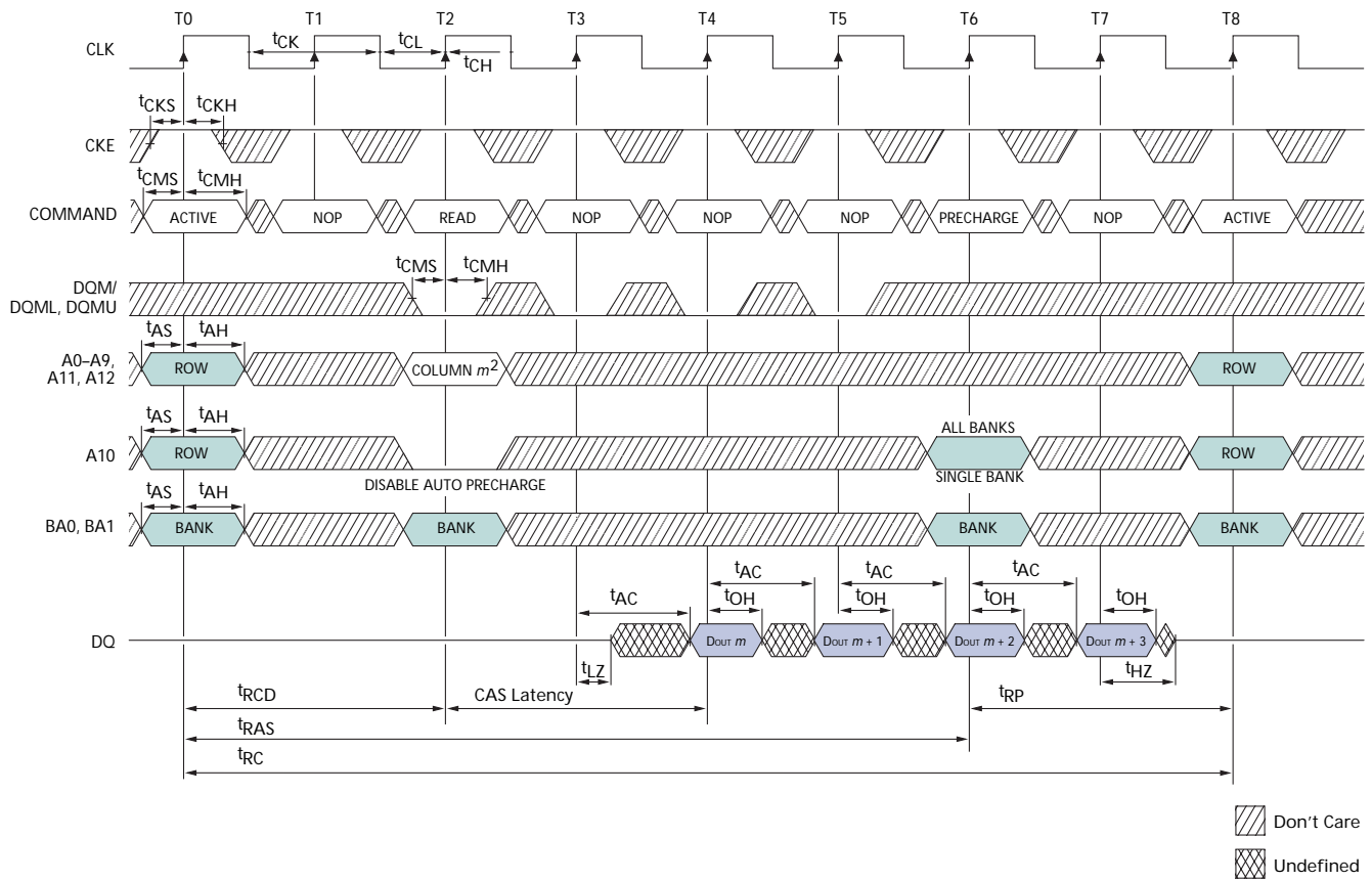
Figure 37: READ – Without Auto Precharge
