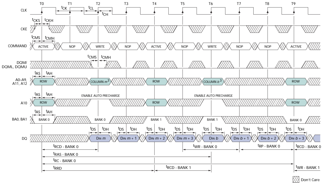
Figure 48: Alternating Bank WRITE Accesses
