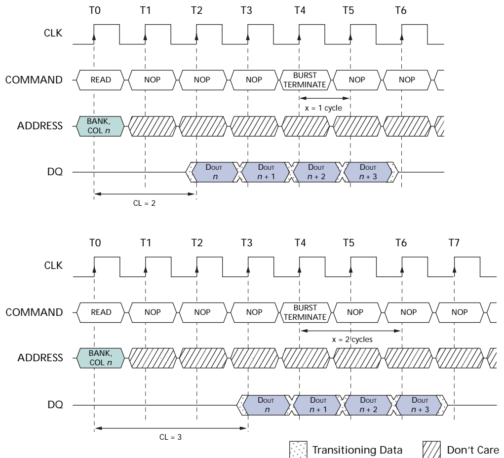
Figure 15: Terminating a READ Burst
