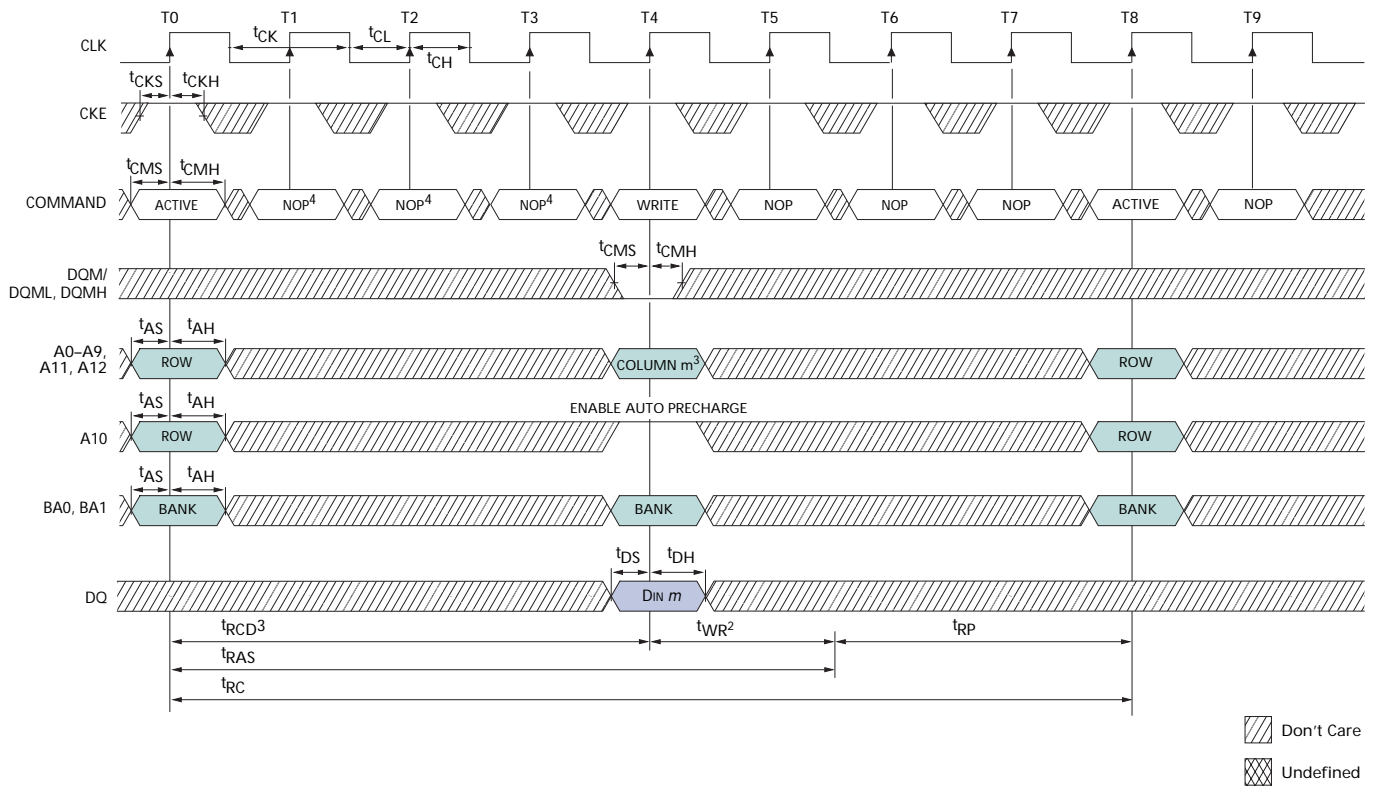
Figure 47: Single WRITE with Auto Precharge
