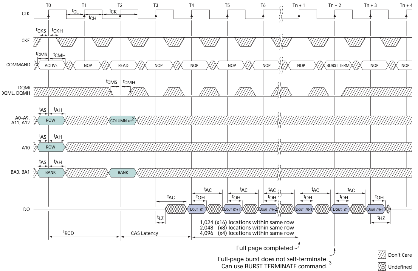
Figure 42: READ – Full-Page Burst
