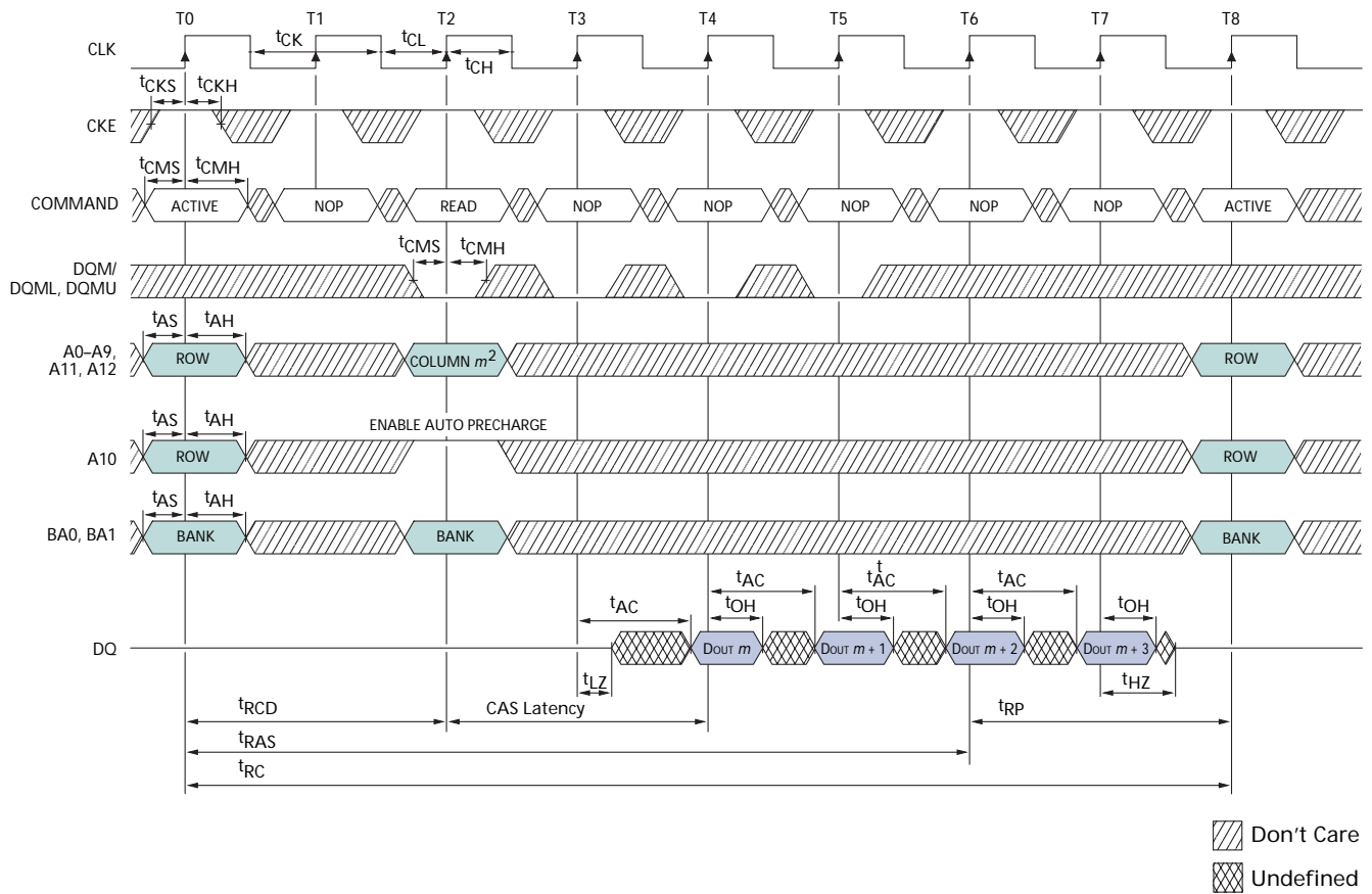
Figure 38: READ – with Auto Precharge
