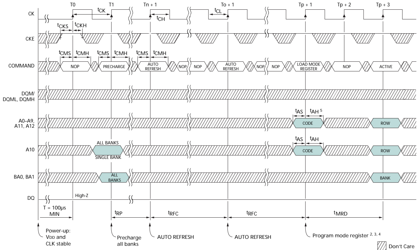
Figure 32: Initialize and Load Mode Register
