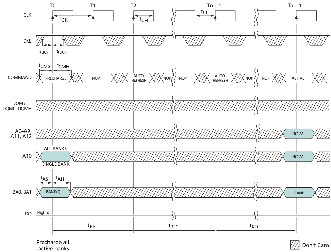
Figure 35: Auto-Refresh Mode
