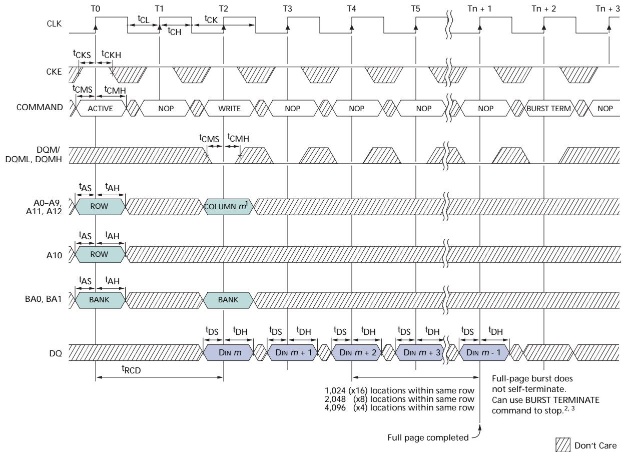
Figure 49: WRITE – Full-Page Burst
