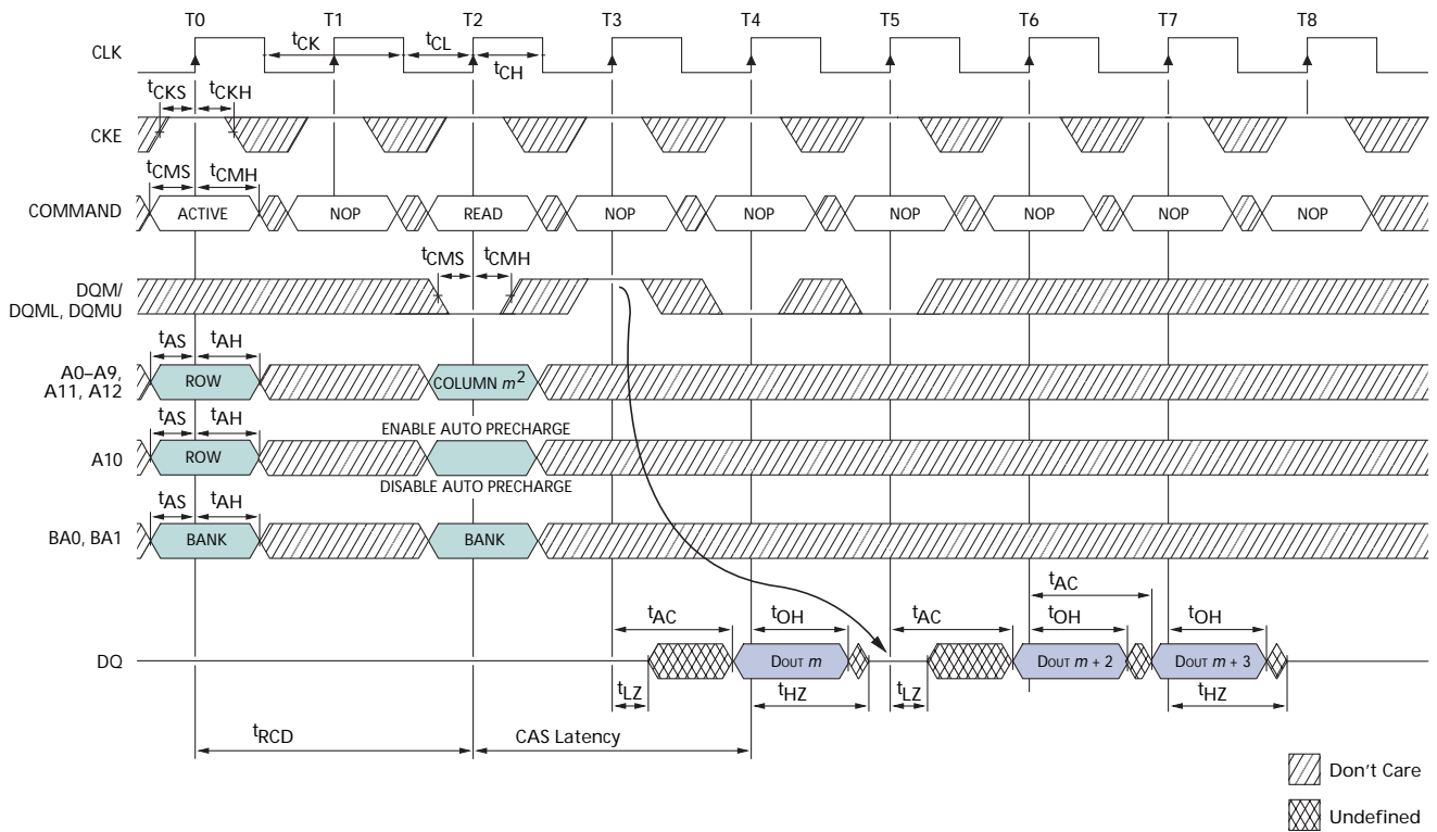
Figure 50: WRITE - DQM Operation
