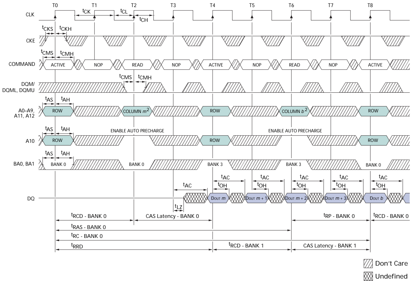
Figure 41: Alternating Bank Read Accesses
