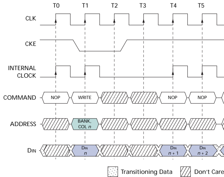
Figure 25: CLOCK SUSPEND During WRITE Burst
