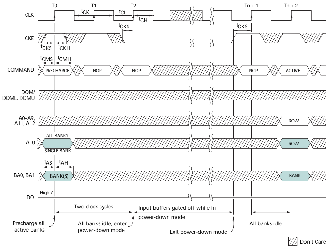
Figure 33: Power-Down Mode
