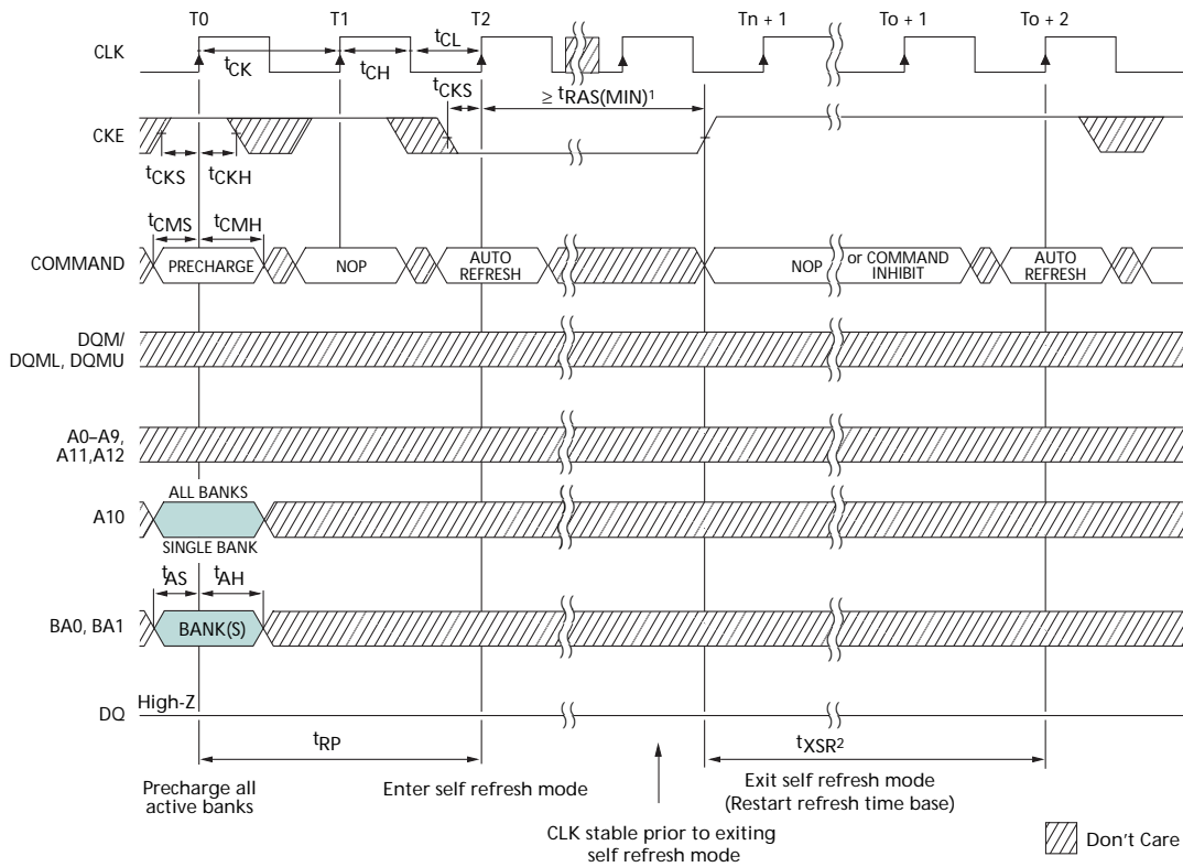
Figure 36: Self-Refresh Mode
