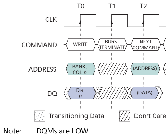
Figure 22: Terminating a WRITE Burst
