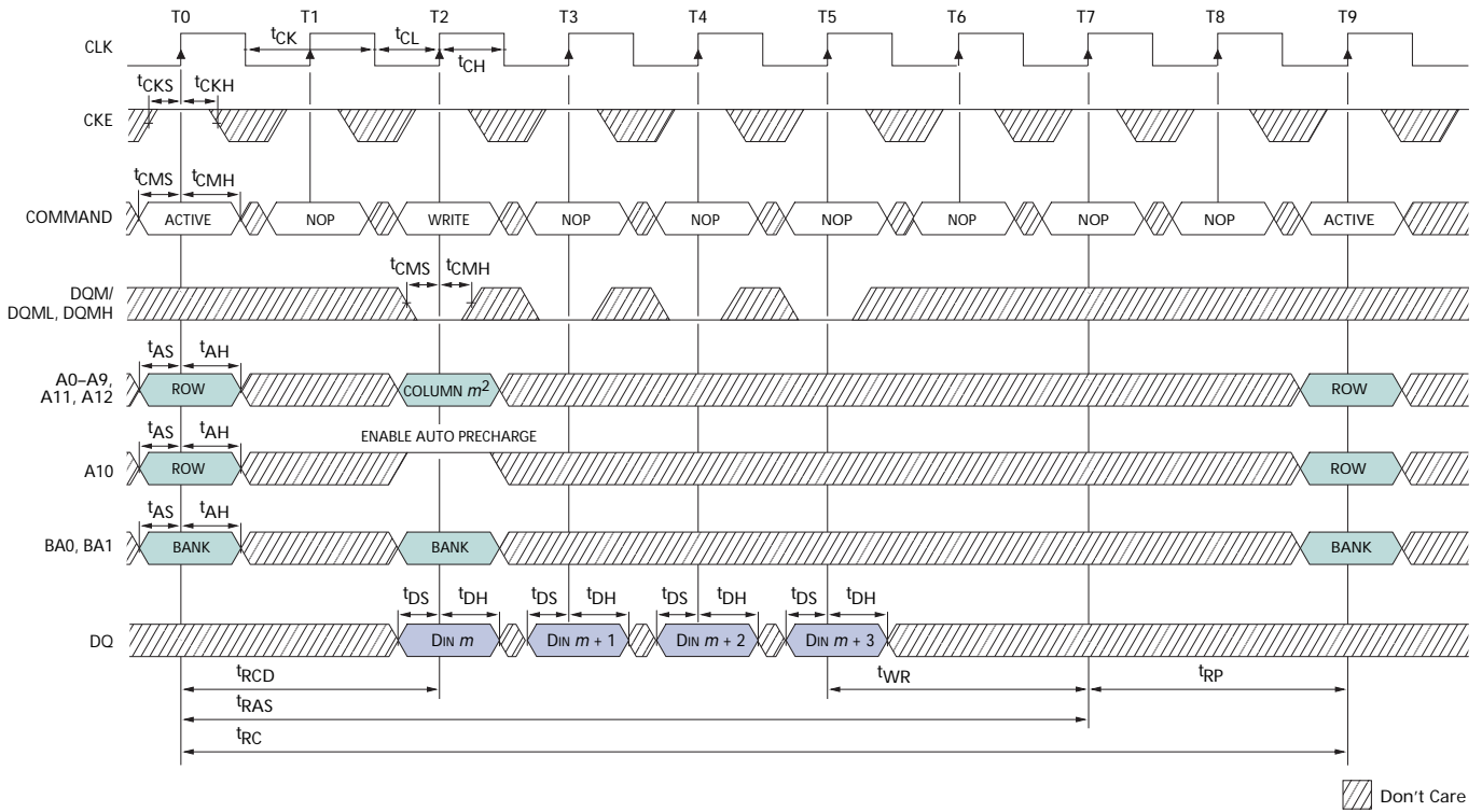
Figure 45: WRITE - with Auto Precharge
