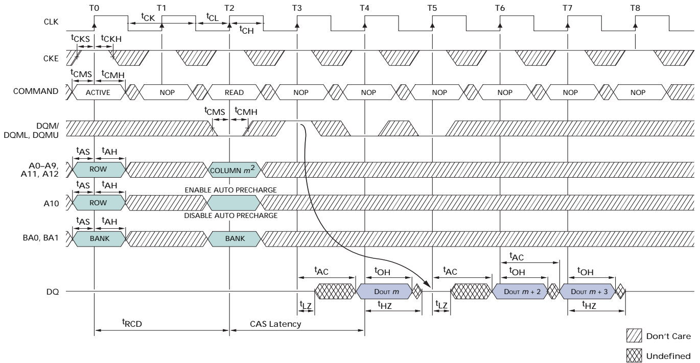
Figure 43: READ DQM Operation
