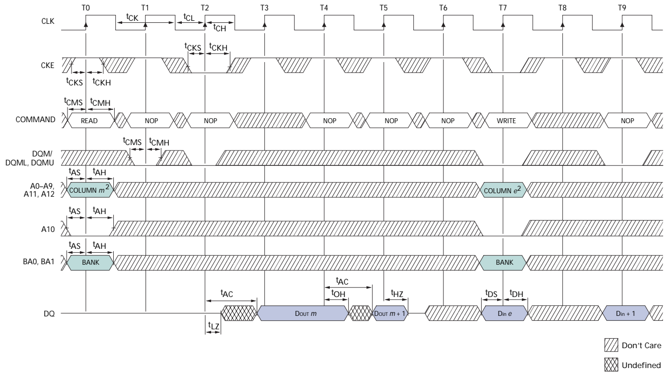
Figure 34: Clock Suspend Mode
