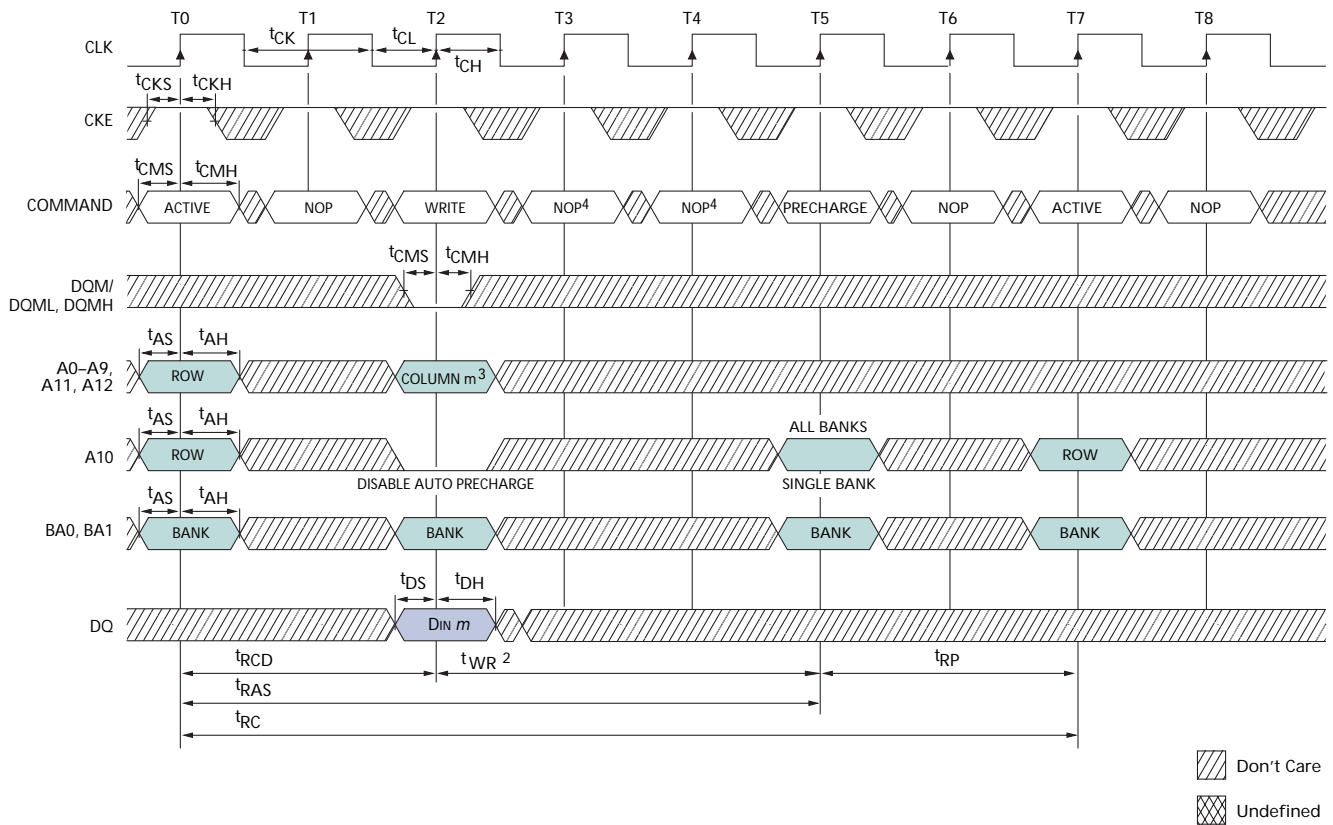
Figure 46: Single WRITE – Without Auto Precharge
