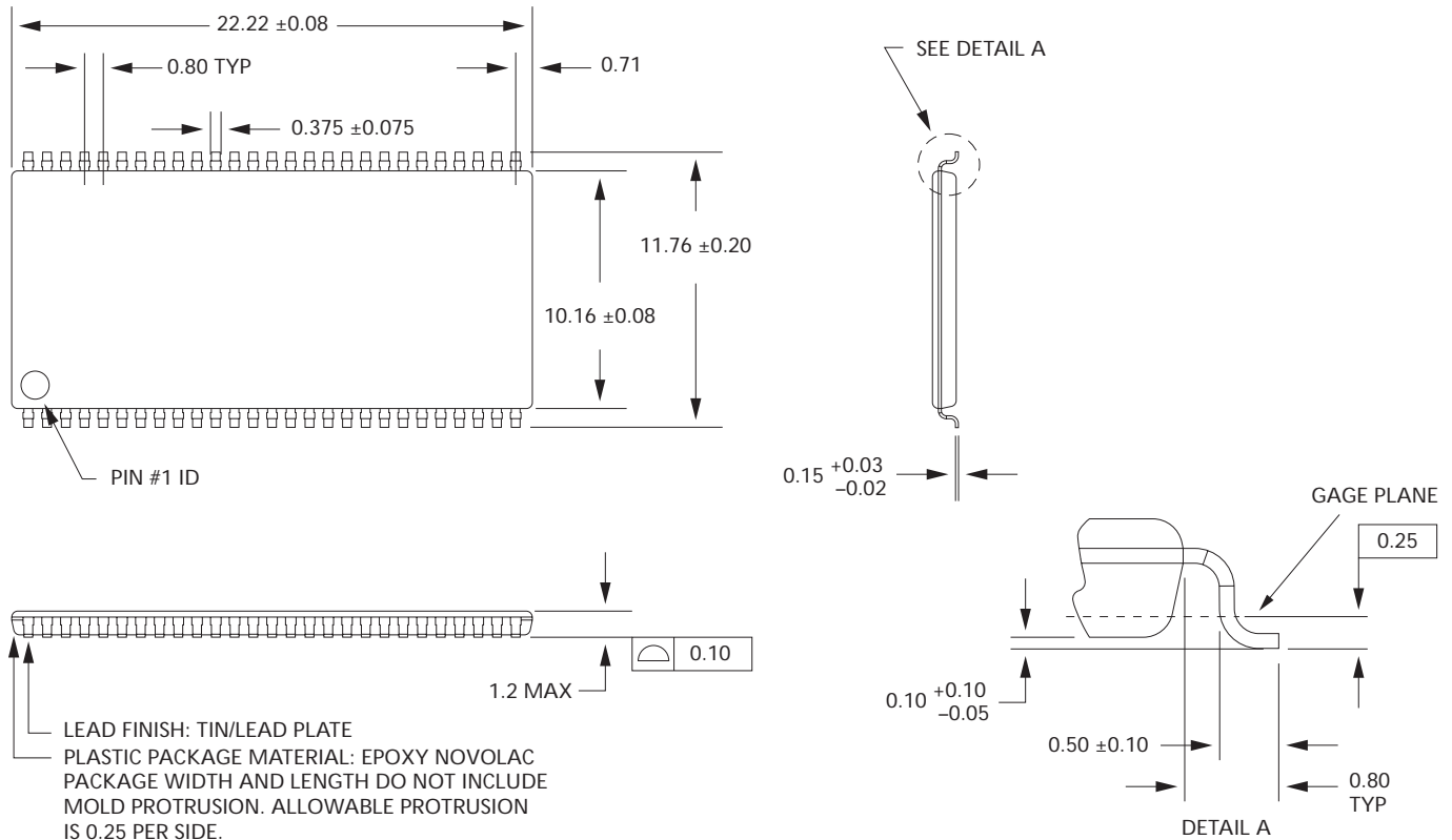
Figure 51: 54-Pin Plastic TSOP (400 mil)
