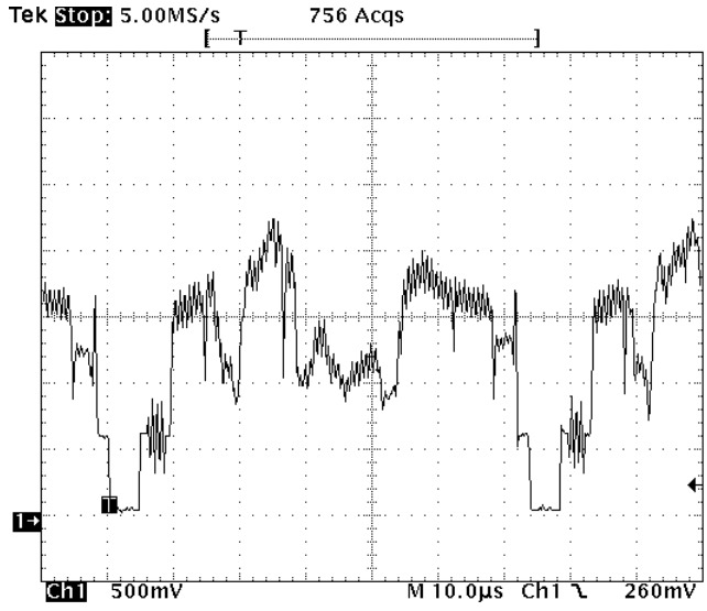
NTSC VIDEO LINE
