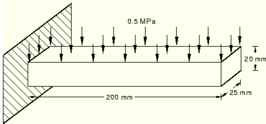
Figure B-1 A loaded cantilever beam.
