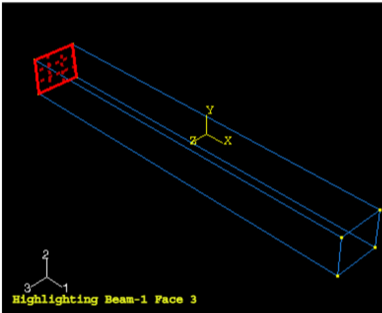
Figure B-9 Selecting the region on which to apply a boundary condition.
